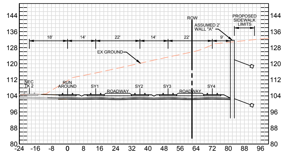
SECTION A-A WEST OF 9TH STREET BRIDGE
