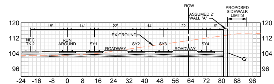
SECTION D-D NORTH YARD
