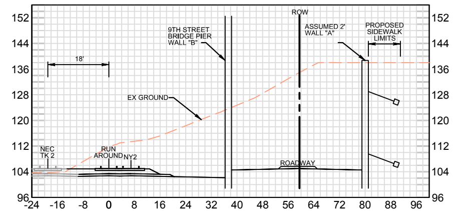
SECTION C-C BELOW 9TH STREET BRIDGE
