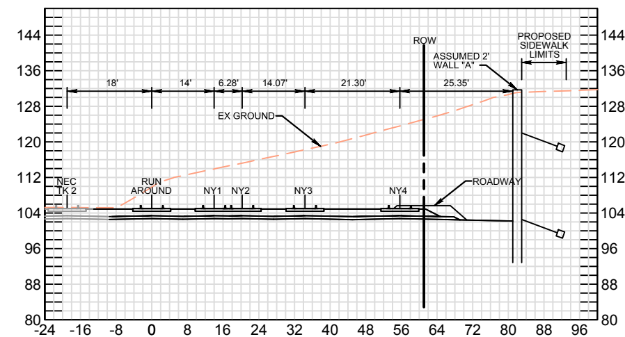
SECTION B-B EAST OF 9TH STREET BRIDGE
