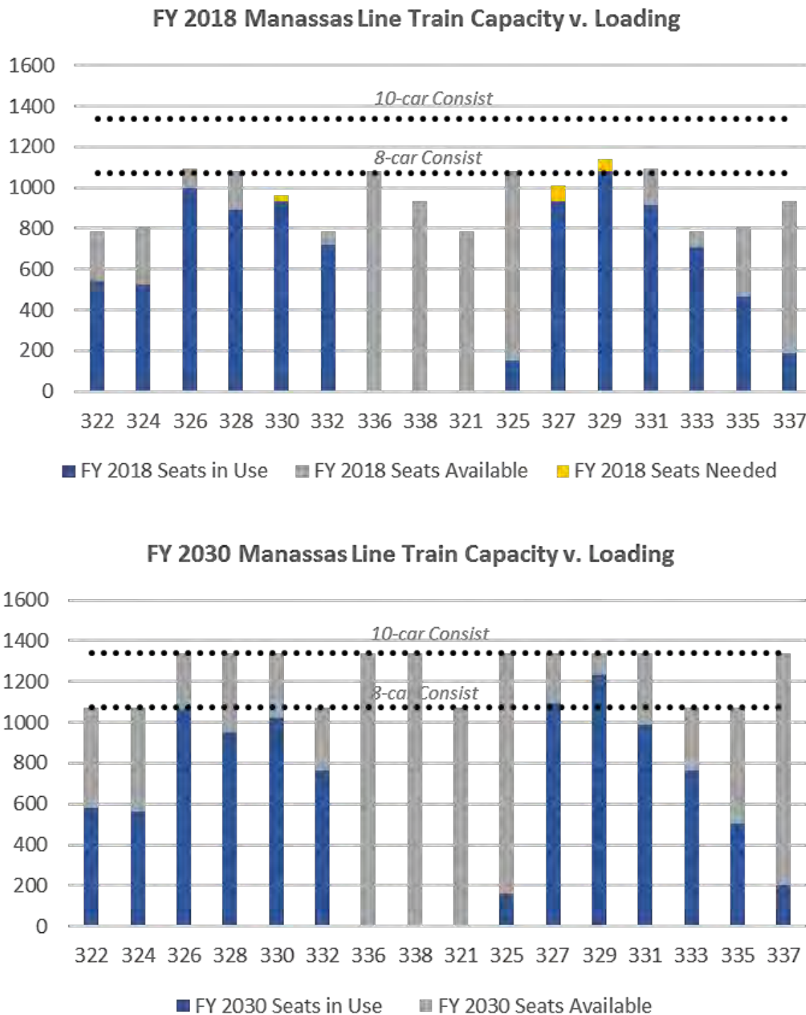
Figure 4-7. Manassas Line FY2018 and FY2030 Train Capacity
